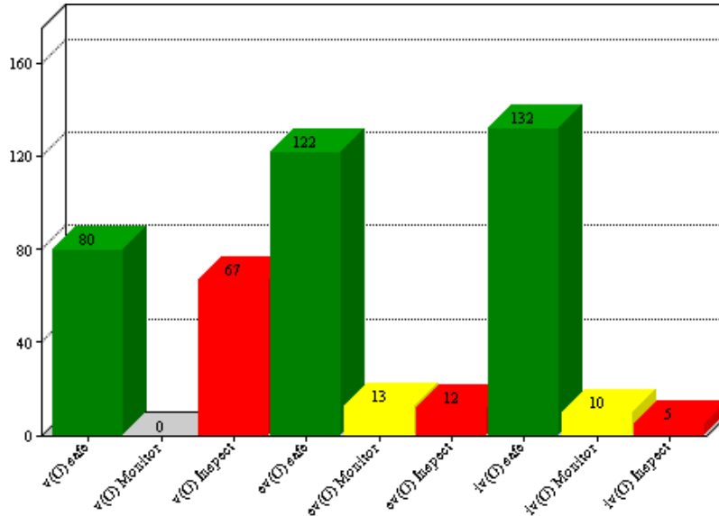
Figure 2: McCabe Metrics Quality Gates
